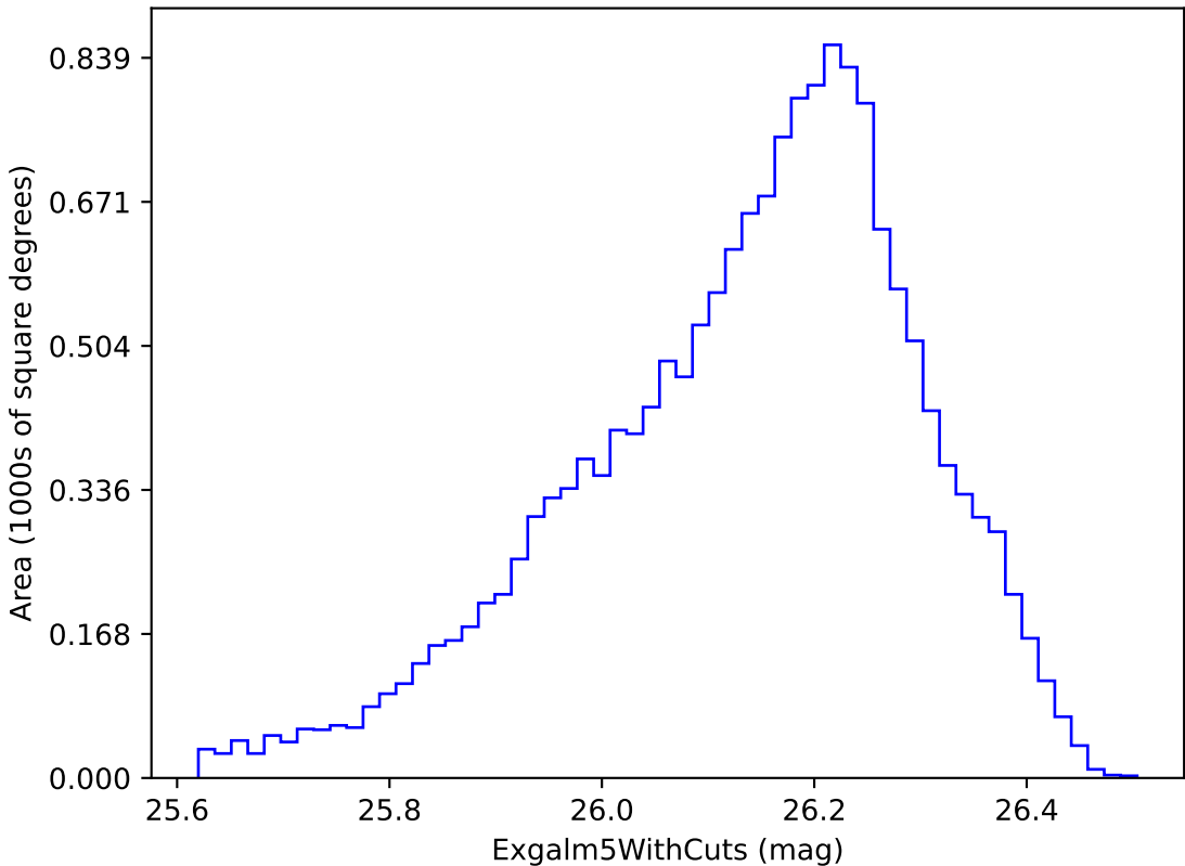
baseline_v3.3_10yrs i band non-DD year 6: ExgalM5WithCuts
