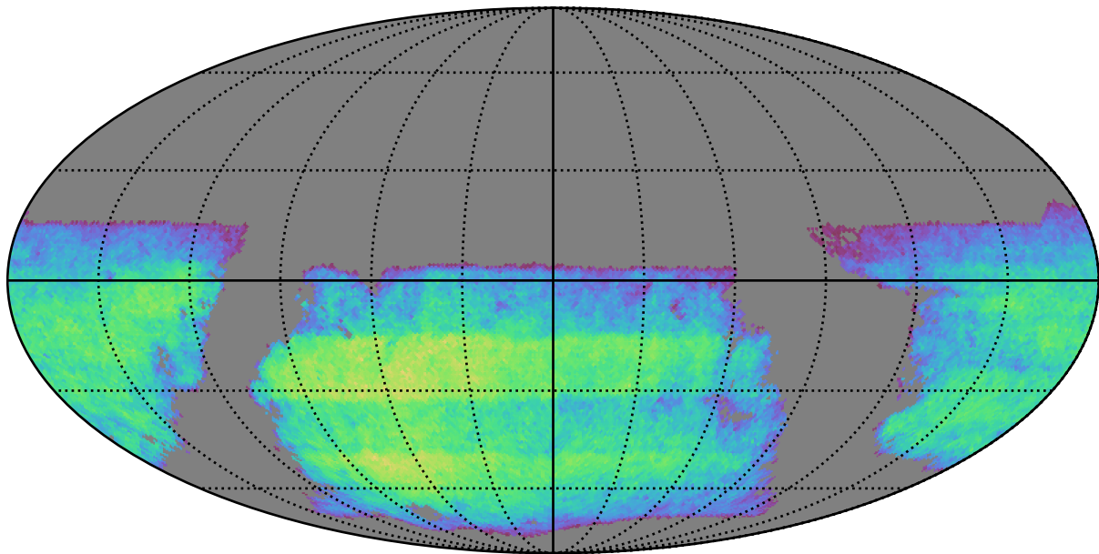
baseline_v3.3_10yrs i band non-DD year 5: ExgalM5WithCuts
