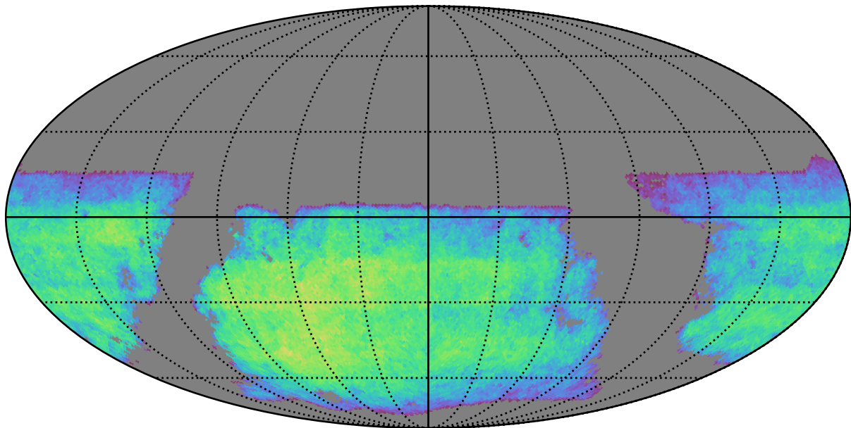
baseline_v3.3_10yrs i band non-DD year 4: ExgalM5WithCuts
