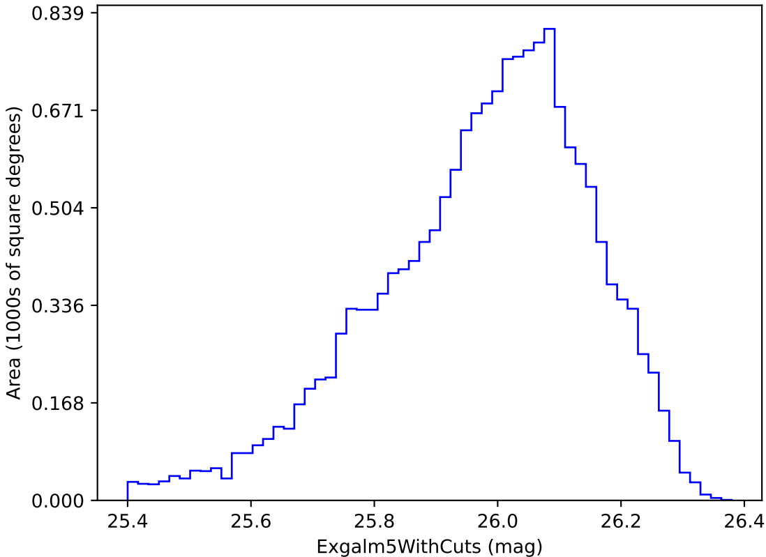
baseline_v3.3_10yrs i band non-DD year 4: ExgalM5WithCuts
