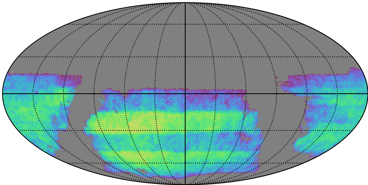
baseline_v3.3_10yrs i band non-DD year 3: ExgalM5WithCuts
