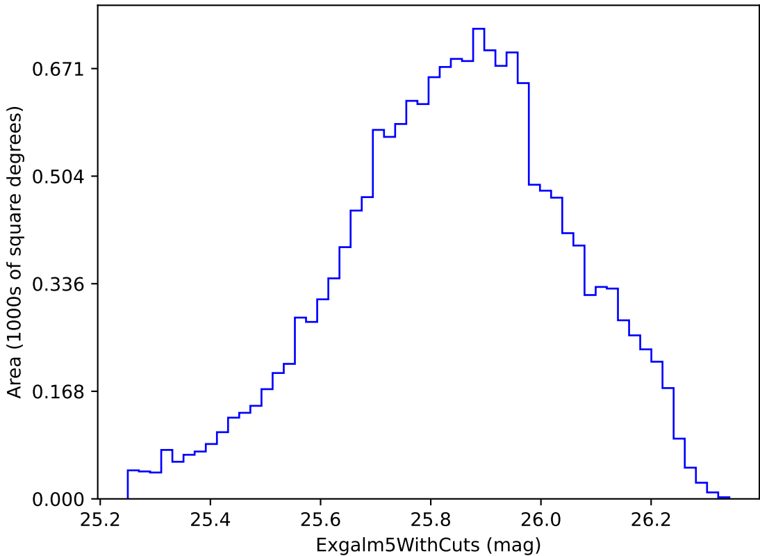
baseline_v3.3_10yrs i band non-DD year 3: ExgalM5WithCuts
