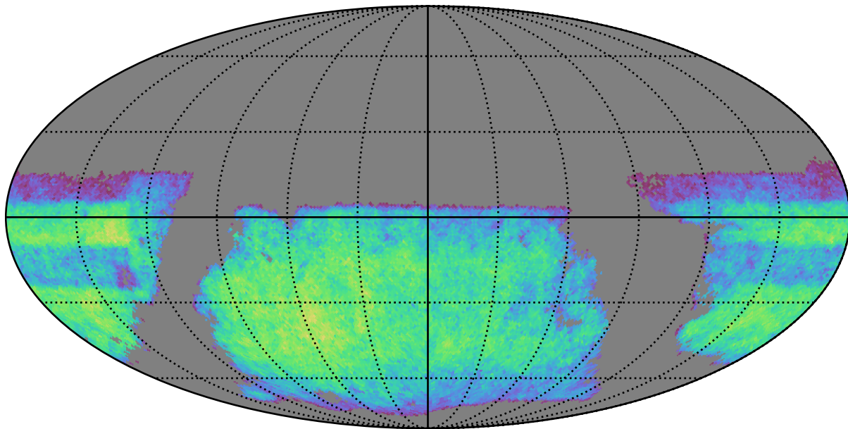
baseline_v3.3_10yrs i band non-DD year 2: ExgalM5WithCuts
