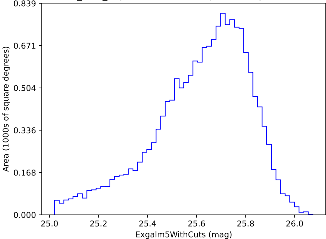
baseline_v3.3_10yrs i band non-DD year 2: ExgalM5WithCuts
