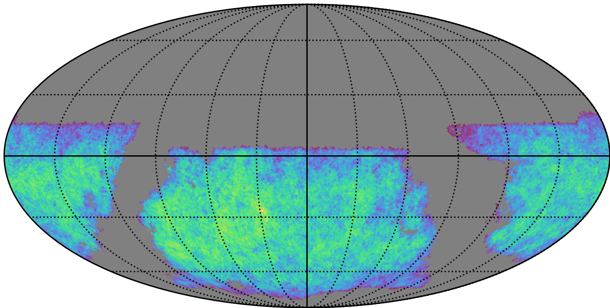
baseline_v3.3_10yrs i band non-DD year 1: ExgalM5WithCuts
