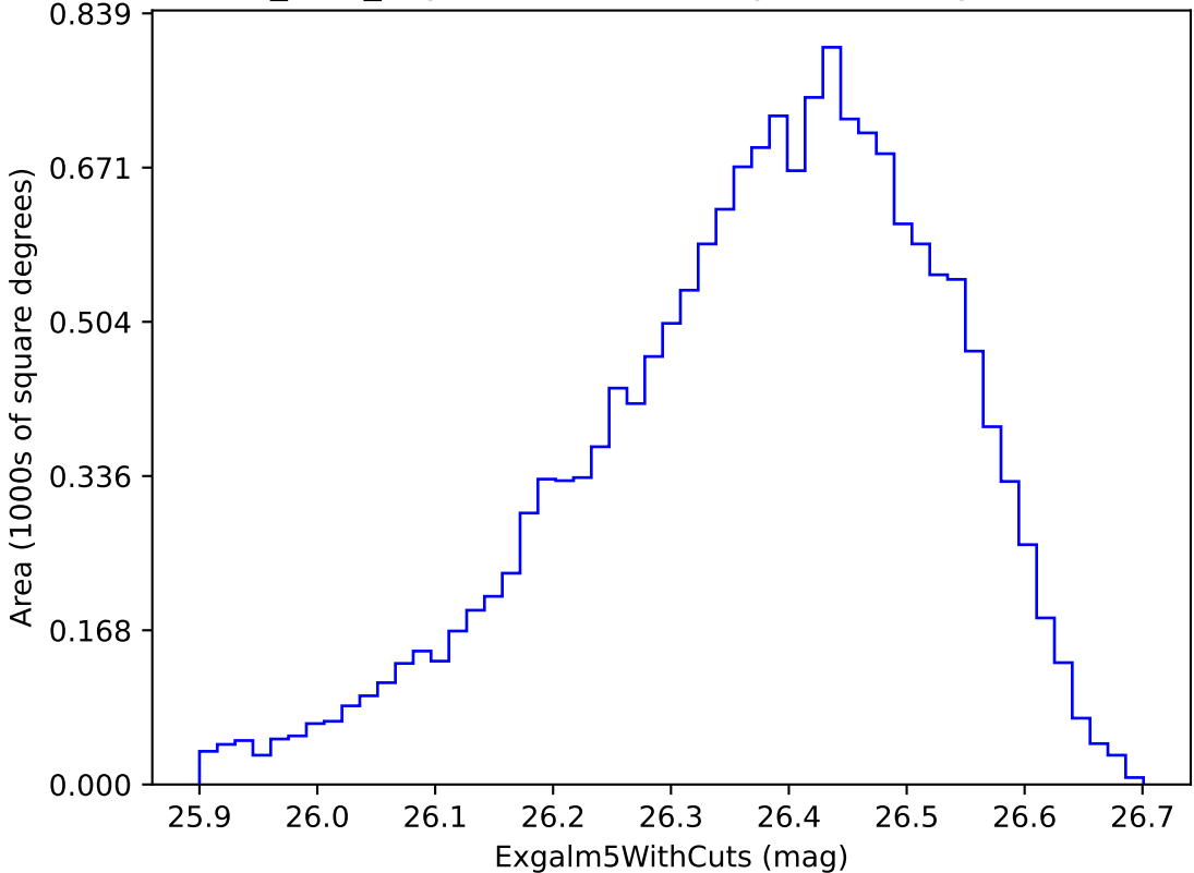
baseline_v3.3_10yrs i band non-DD year 10: ExgalM5WithCuts
