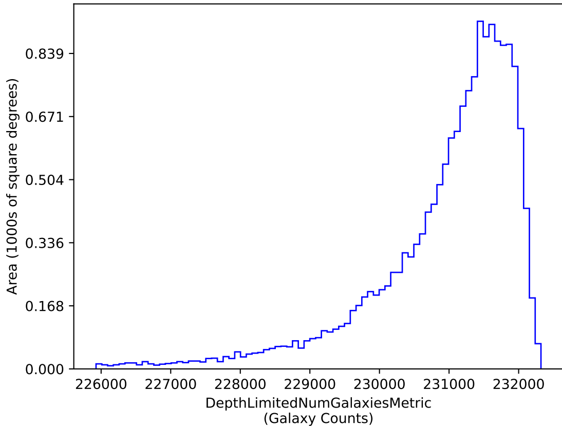
baseline_v3.3_10yrs i band galaxies non-DD: DepthLimitedNumGalaxiesMetric
