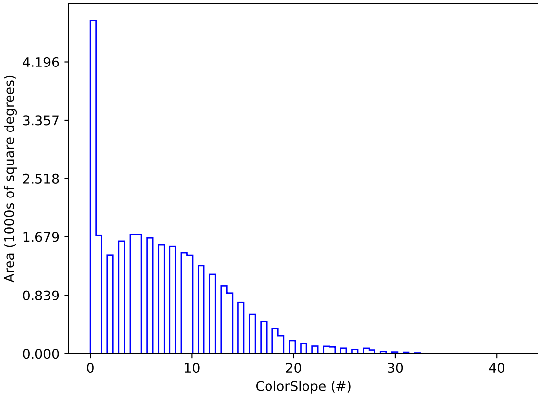
baseline_v3.3_10yrs visitExposureTime > 19: ColorSlope
