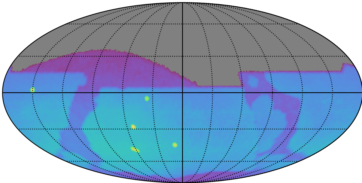
baseline_v3.3_10yrs : Brown Dwarf, L7
