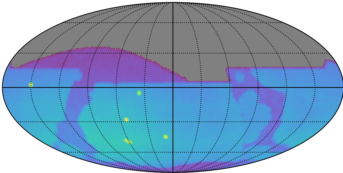
baseline_v3.3_10yrs : Brown Dwarf, L4
