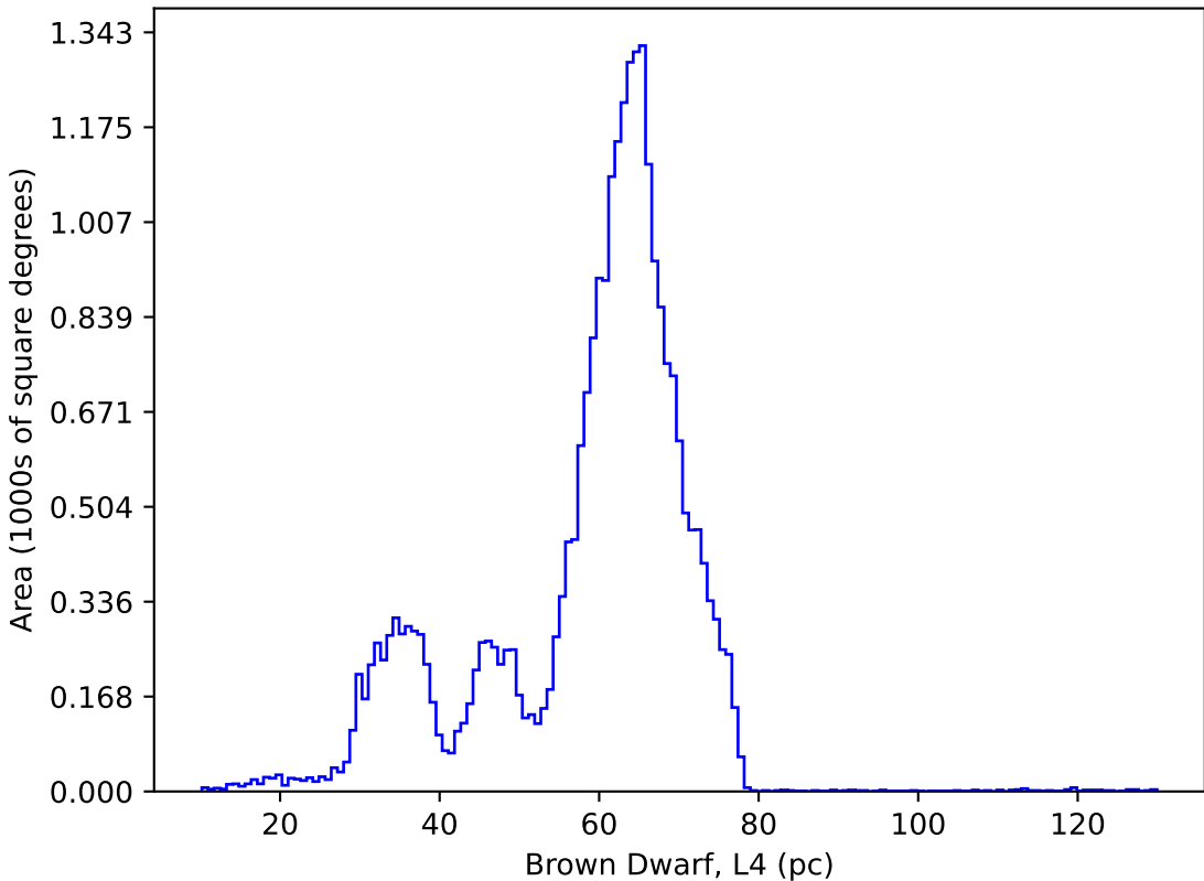
baseline_v3.3_10yrs : Brown Dwarf, L4
