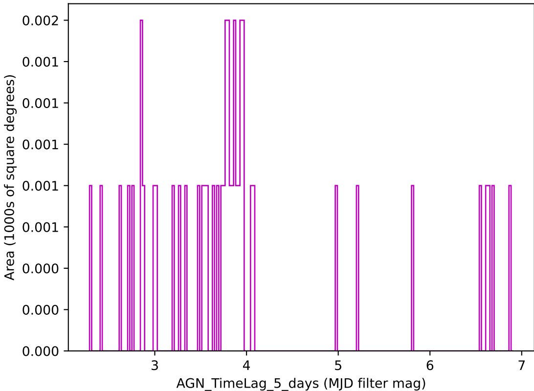
baseline_v3.3_10yrs z band: AGN_TimeLag_5_days
