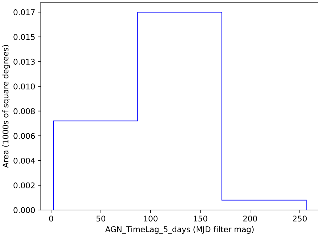
baseline_v3.3_10yrs y band: AGN_TimeLag_5_days
