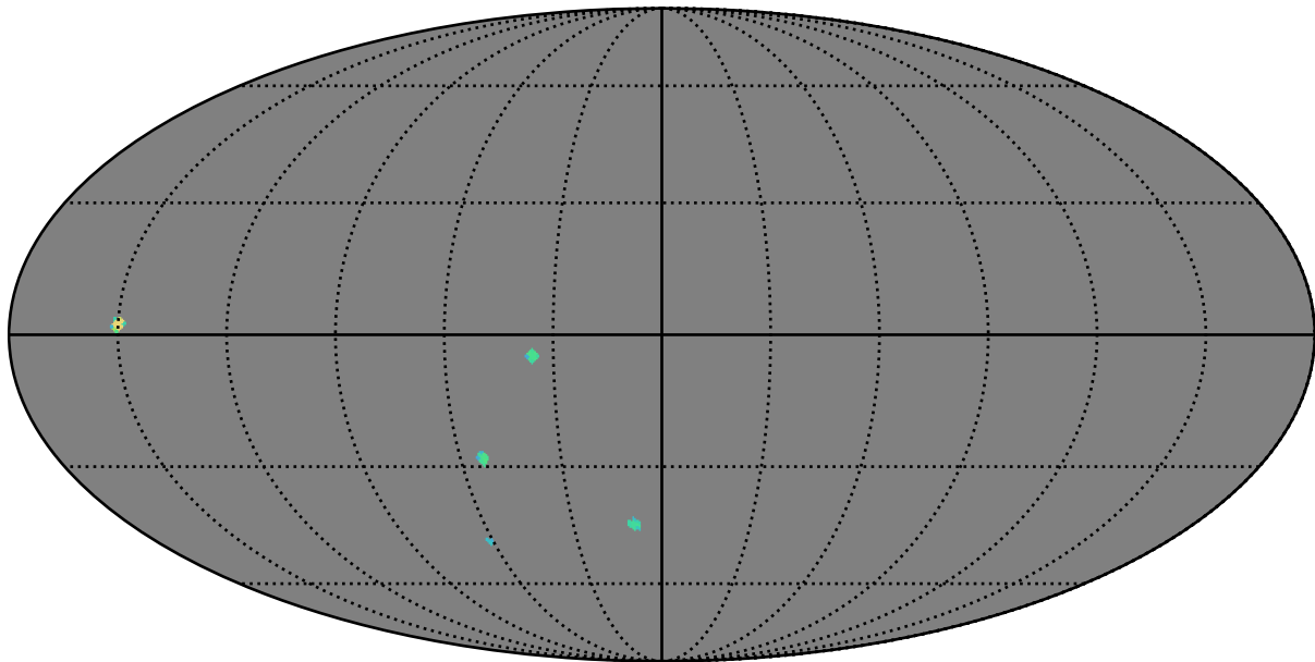
baseline_v3.3_10yrs r band: AGN_TimeLag_5_days
