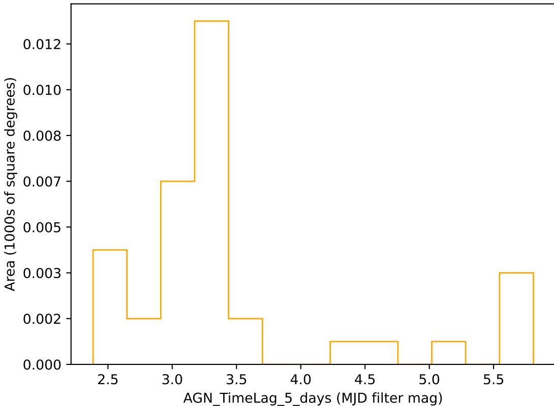
baseline_v3.3_10yrs r band: AGN_TimeLag_5_days
