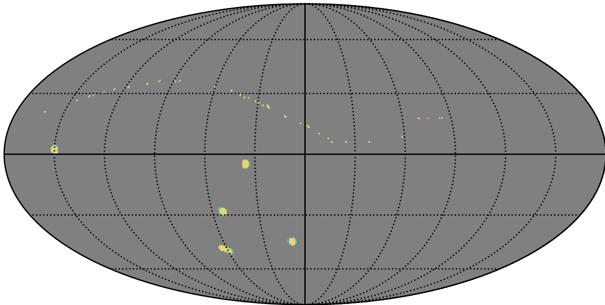
baseline_v3.3_10yrs all bands: AGN_TimeLag_5_days
