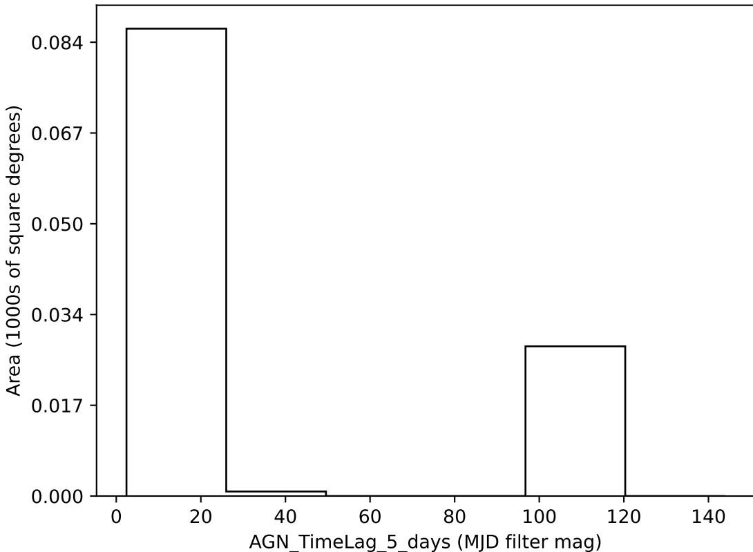
baseline_v3.3_10yrs all bands: AGN_TimeLag_5_days
