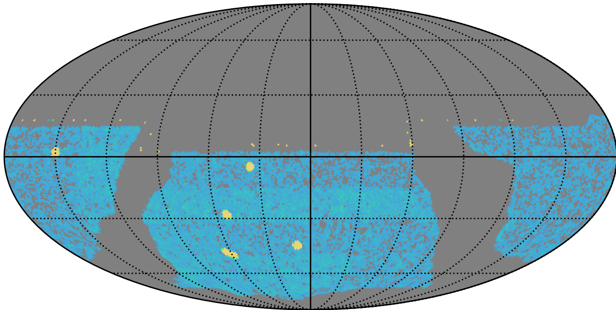
baseline_v3.3_10yrs y band: AGN_TimeLag_100_days
