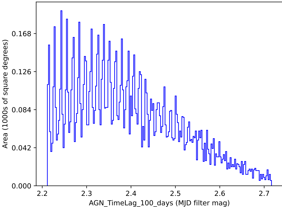
baseline_v3.3_10yrs y band: AGN_TimeLag_100_days
