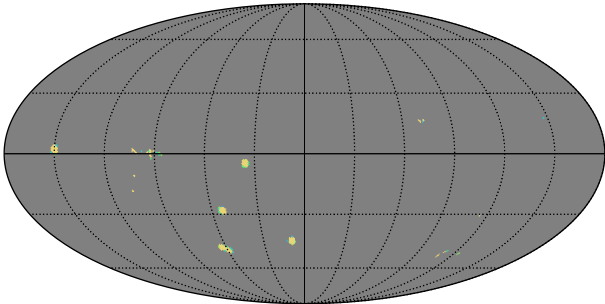
baseline_v3.3_10yrs u band: AGN_TimeLag_100_days
