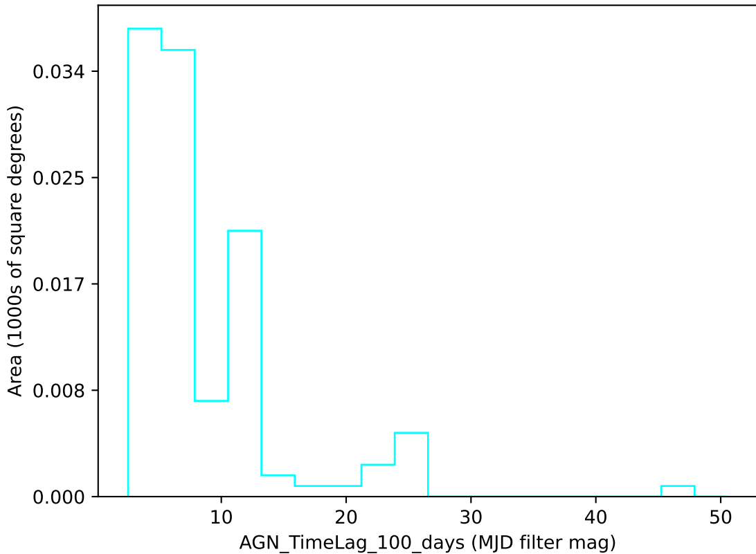
baseline_v3.3_10yrs u band: AGN_TimeLag_100_days
