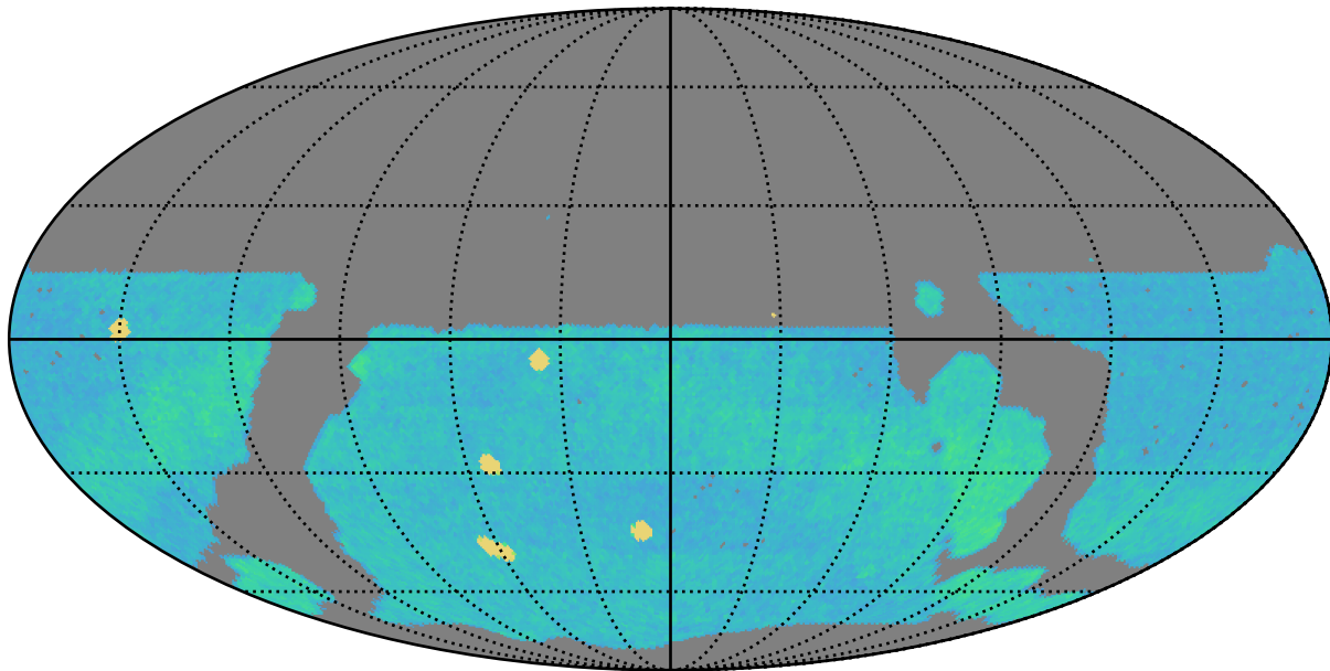
baseline_v3.3_10yrs r band: AGN_TimeLag_100_days
