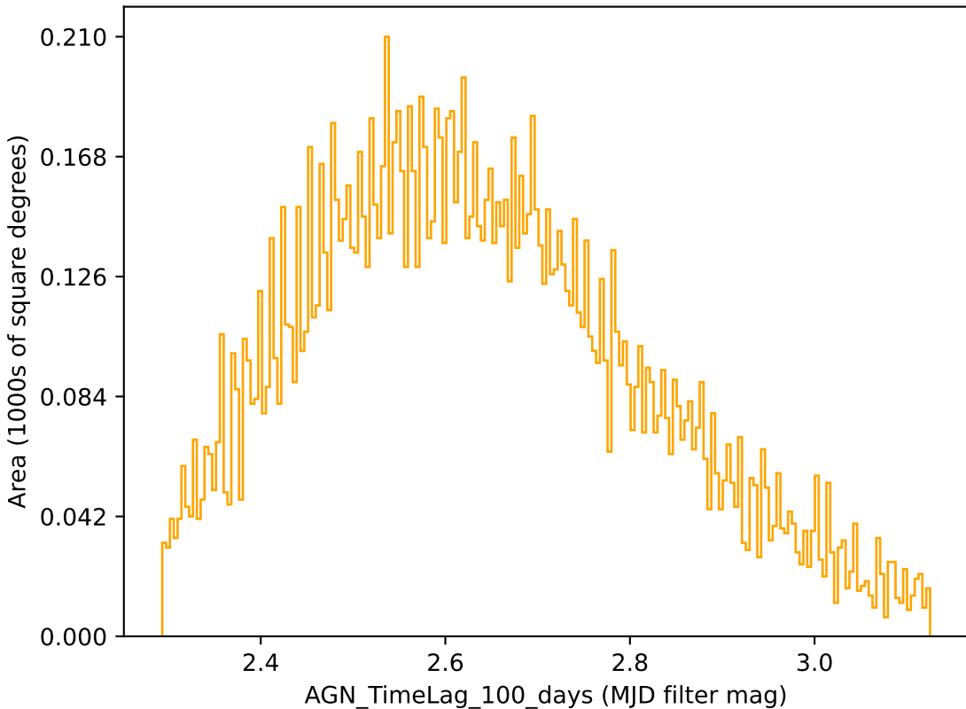
baseline_v3.3_10yrs r band: AGN_TimeLag_100_days
