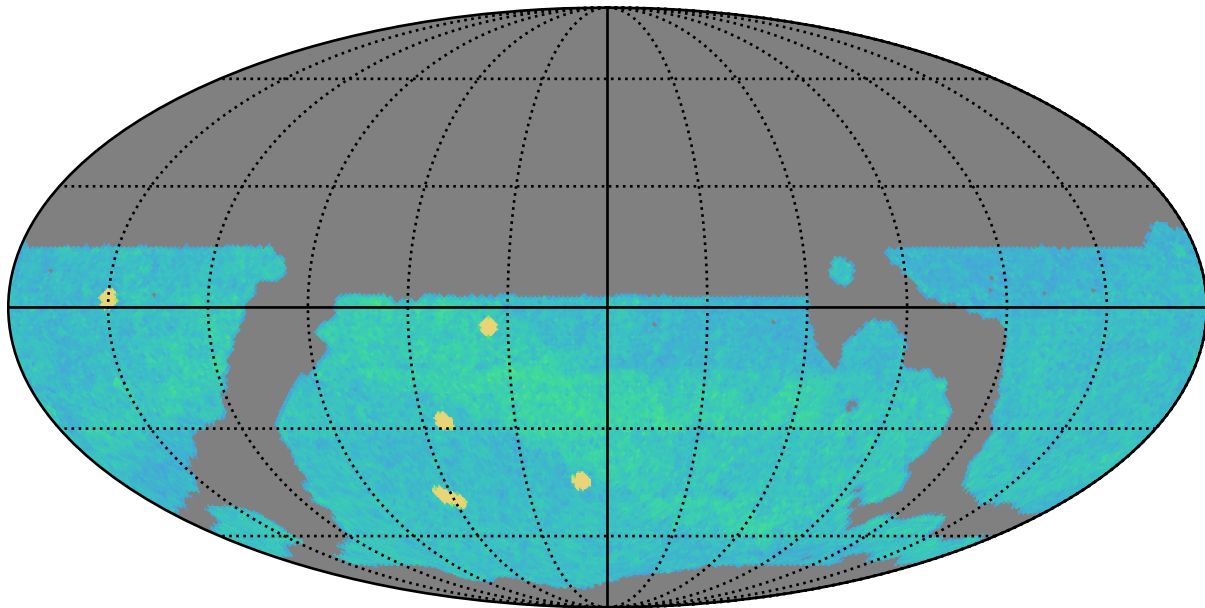
baseline_v3.3_10yrs i band: AGN_TimeLag_100_days
