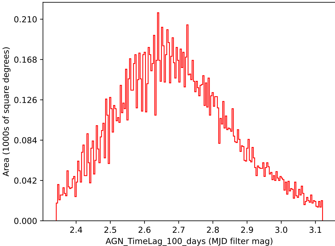
baseline_v3.3_10yrs i band: AGN_TimeLag_100_days
