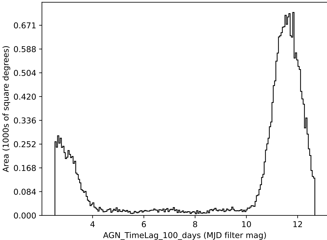
baseline_v3.3_10yrs all bands: AGN_TimeLag_100_days
