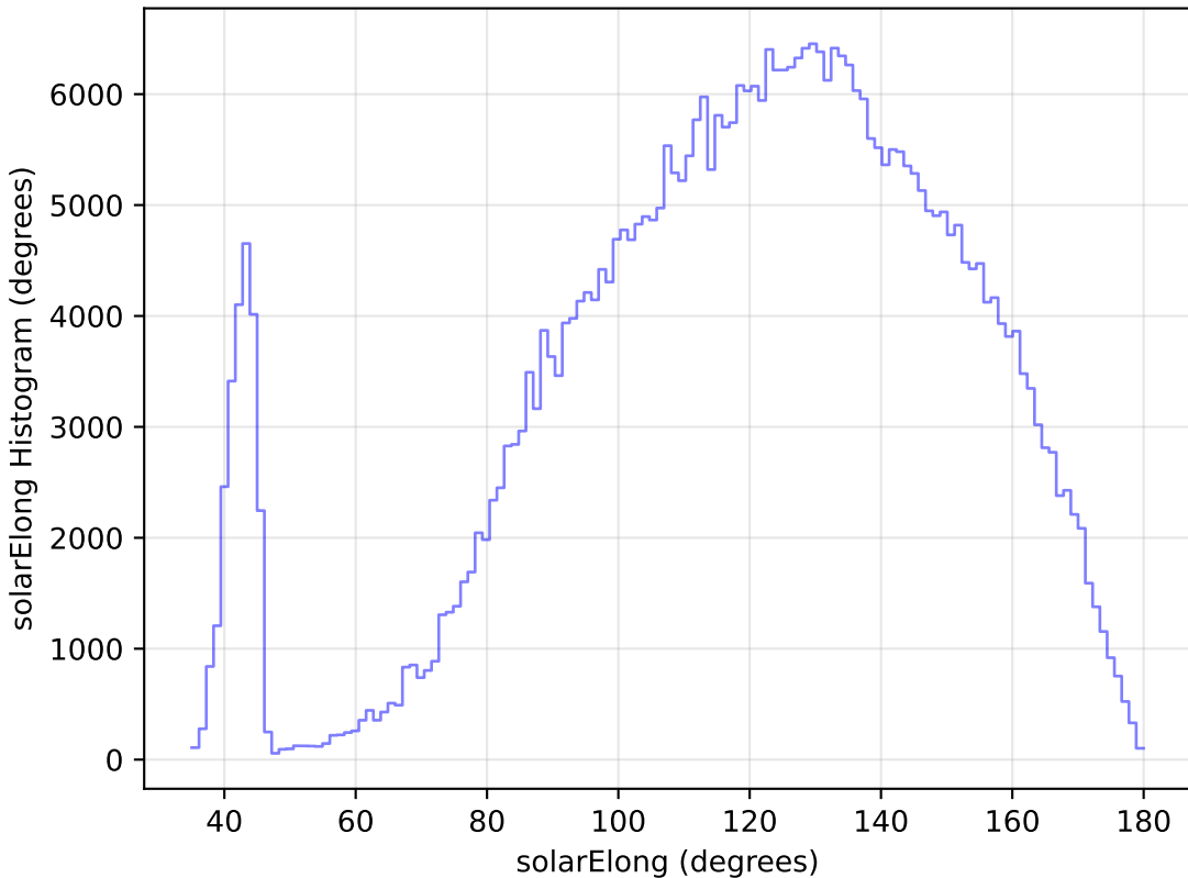
baseline_v3.3_10yrs WFD z band: solarElong Histogram
