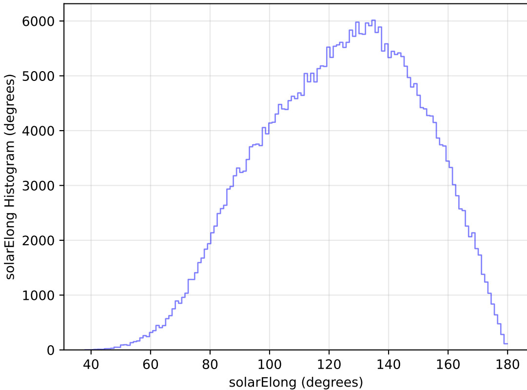
baseline_v3.3_10yrs WFD y band: solarElong Histogram
