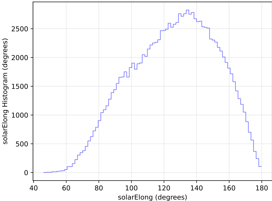
baseline_v3.3_10yrs WFD u band: solarElong Histogram
