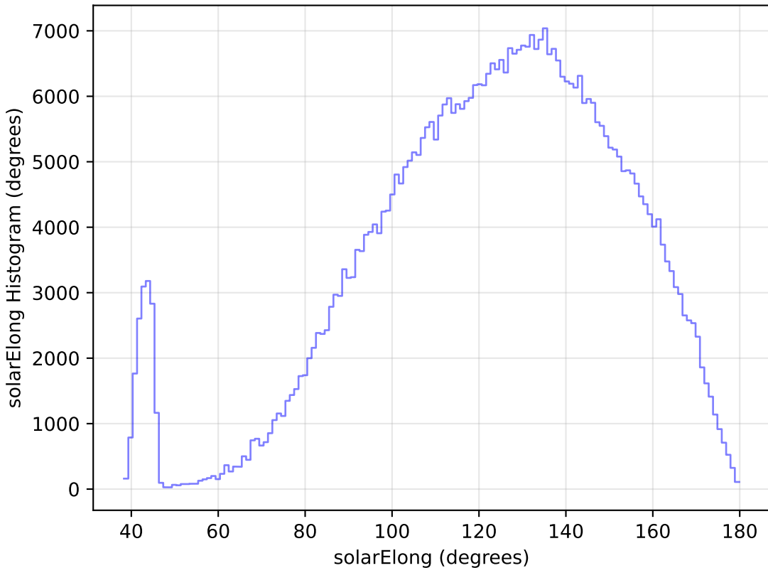
baseline_v3.3_10yrs WFD r band: solarElong Histogram
