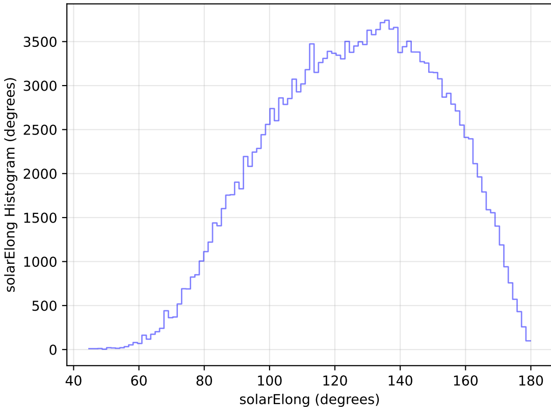
baseline_v3.3_10yrs WFD g band: solarElong Histogram
