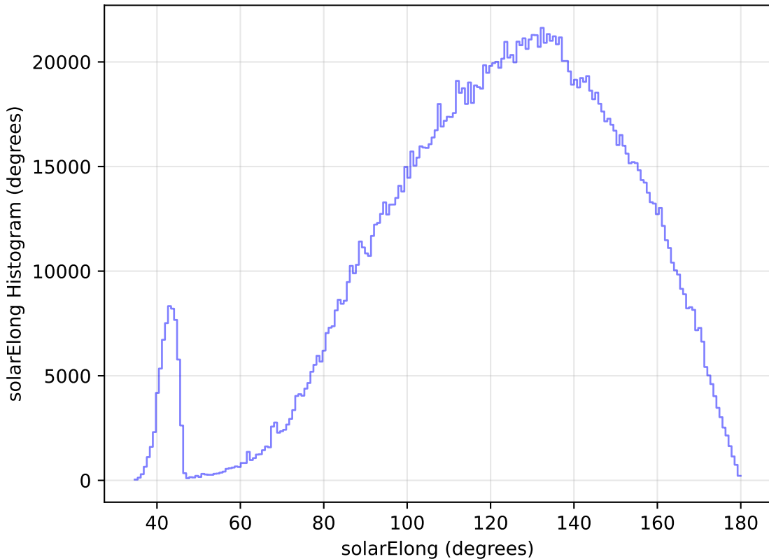
baseline_v3.3_10yrs WFD all bands: solarElong Histogram
