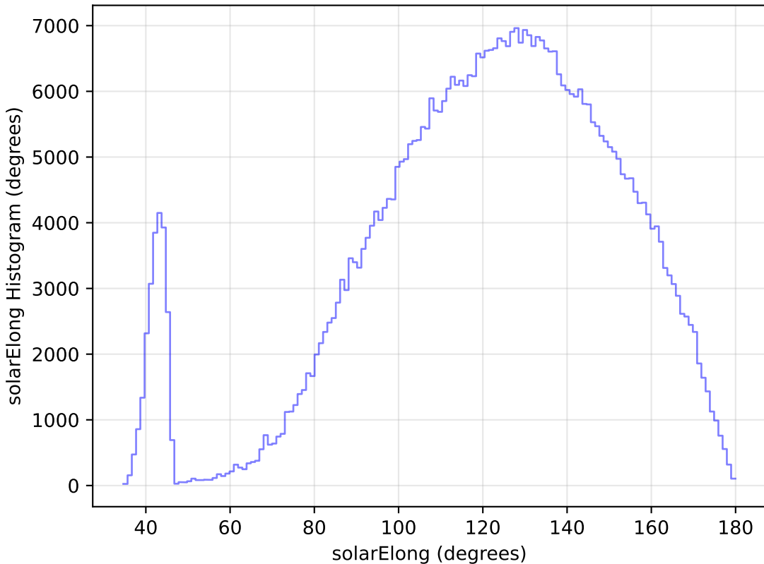
baseline_v3.3_10yrs All sky i band: solarElong Histogram
