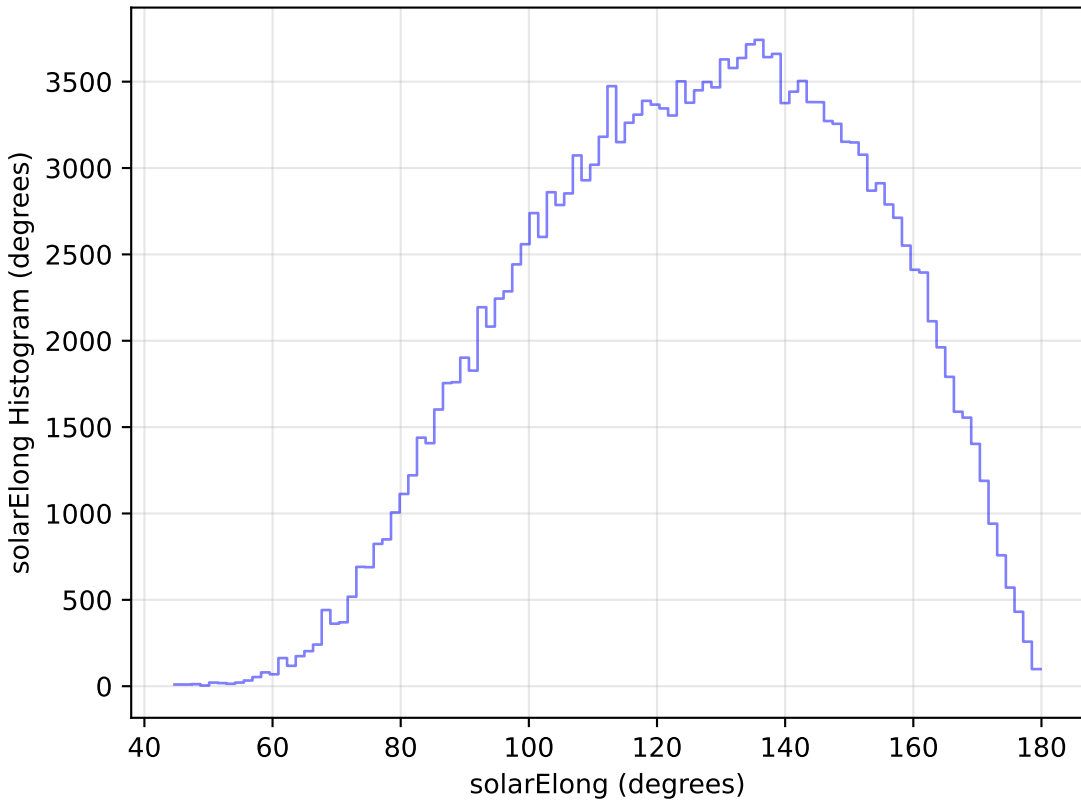
baseline_v3.3_10yrs All sky g band: solarElong Histogram
