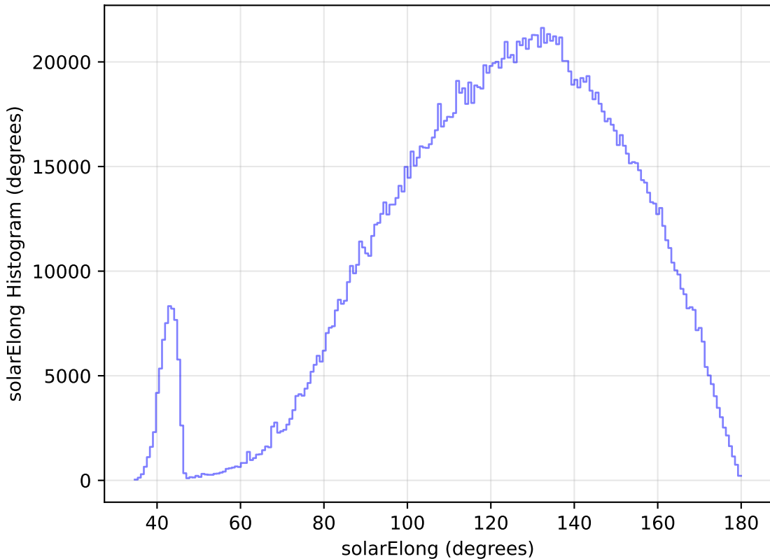
baseline_v3.3_10yrs All sky all bands: solarElong Histogram
