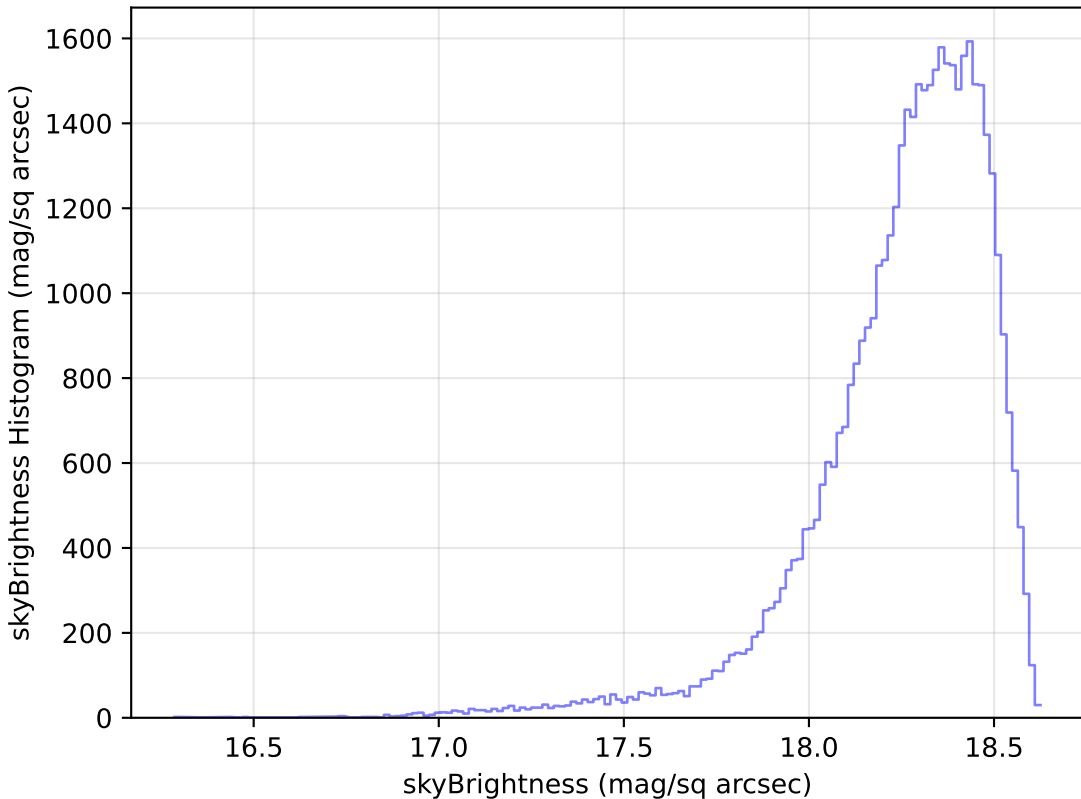
baseline_v3.3_10yrs Yr 1 y band: skyBrightness Histogram
