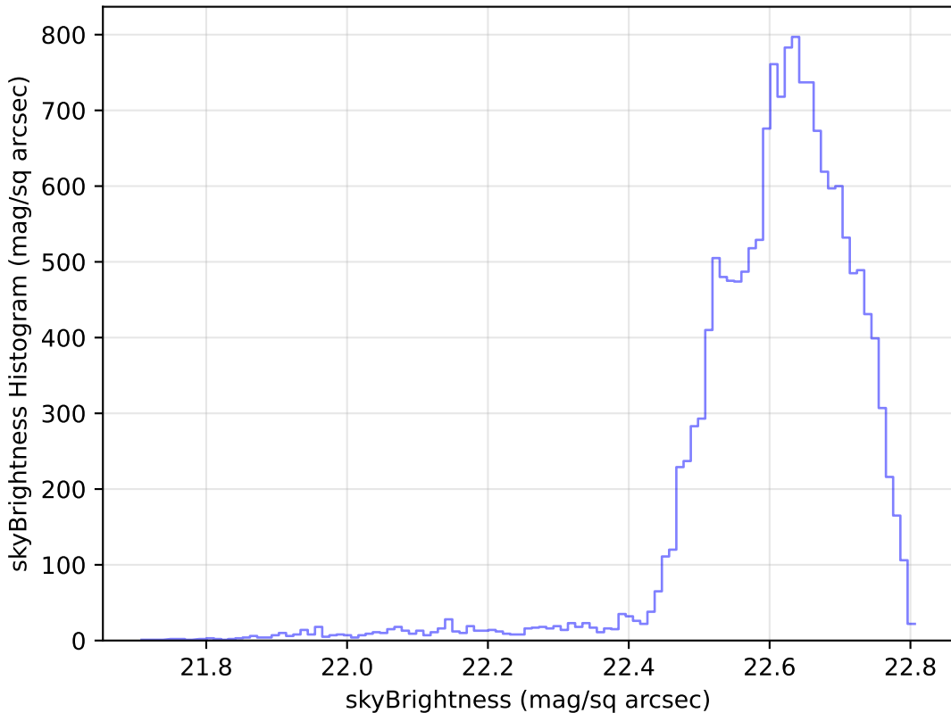
baseline_v3.3_10yrs Yr 1 u band: skyBrightness Histogram
