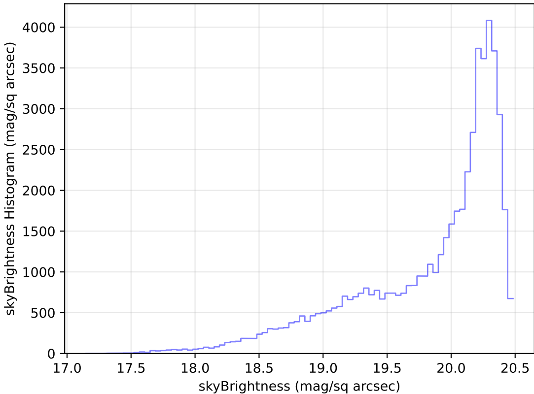
baseline_v3.3_10yrs Yr 1 i band: skyBrightness Histogram
