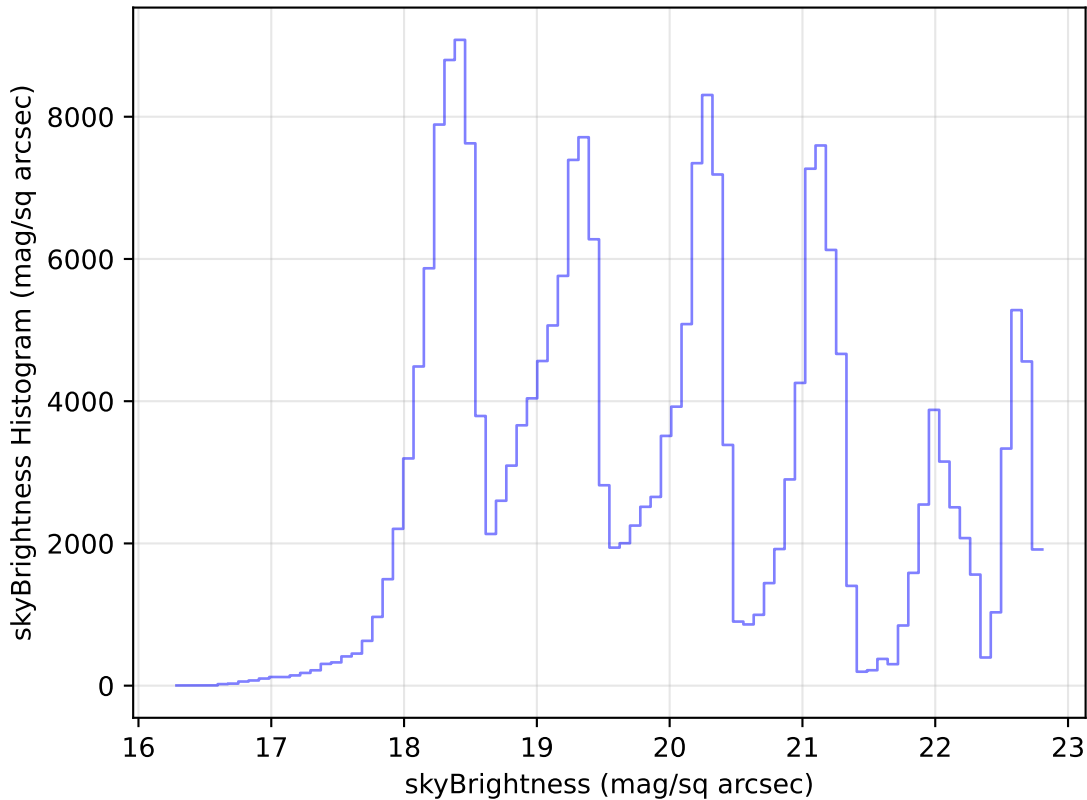
baseline_v3.3_10yrs Yr 1 all bands: skyBrightness Histogram
