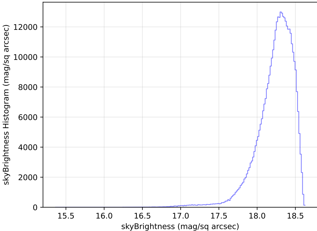
baseline_v3.3_10yrs WFD y band: skyBrightness Histogram
