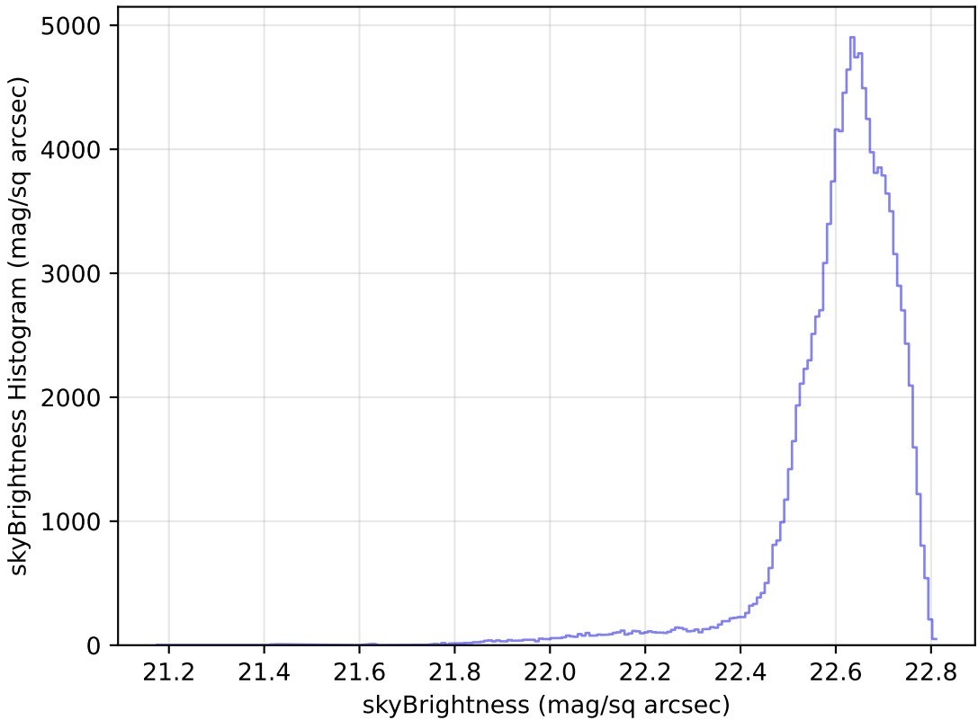
baseline_v3.3_10yrs WFD u band: skyBrightness Histogram
