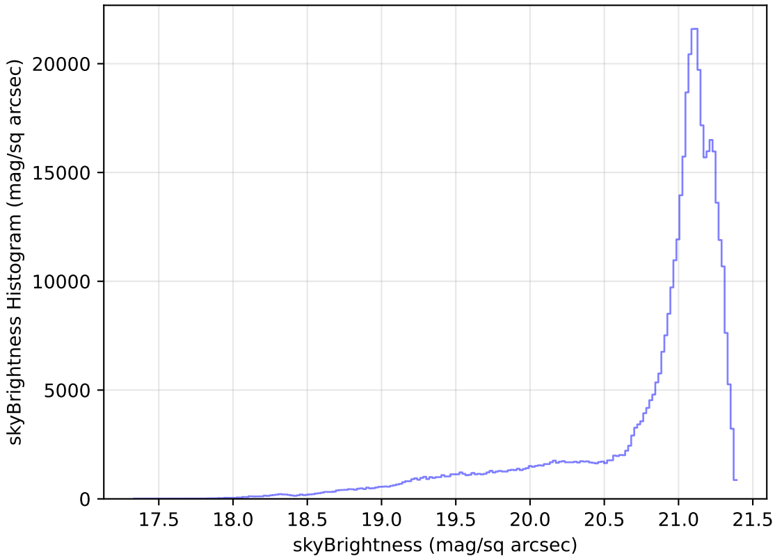
baseline_v3.3_10yrs WFD r band: skyBrightness Histogram
