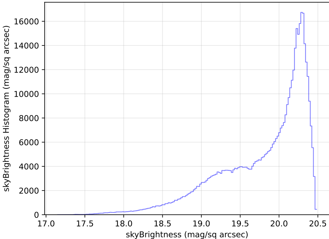
baseline_v3.3_10yrs WFD i band: skyBrightness Histogram
