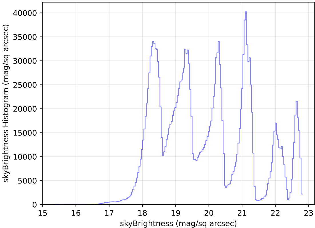
baseline_v3.3_10yrs WFD all bands: skyBrightness Histogram
