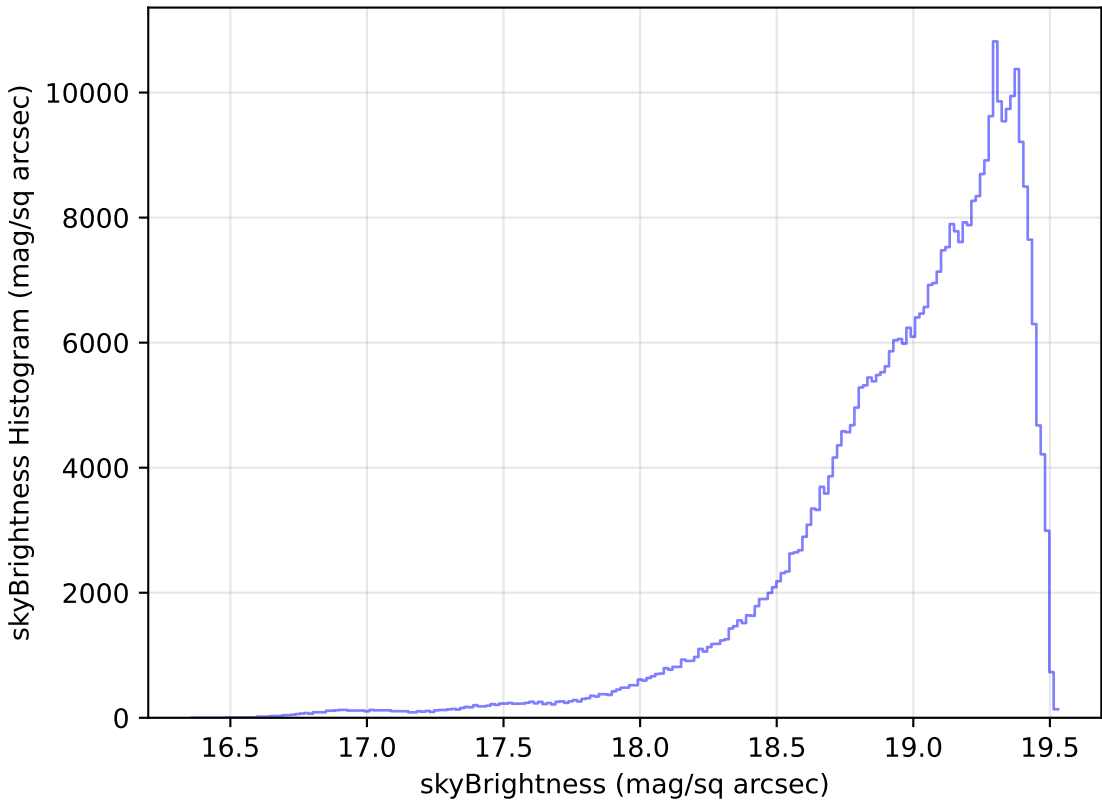
baseline_v3.3_10yrs All sky z band: skyBrightness Histogram
