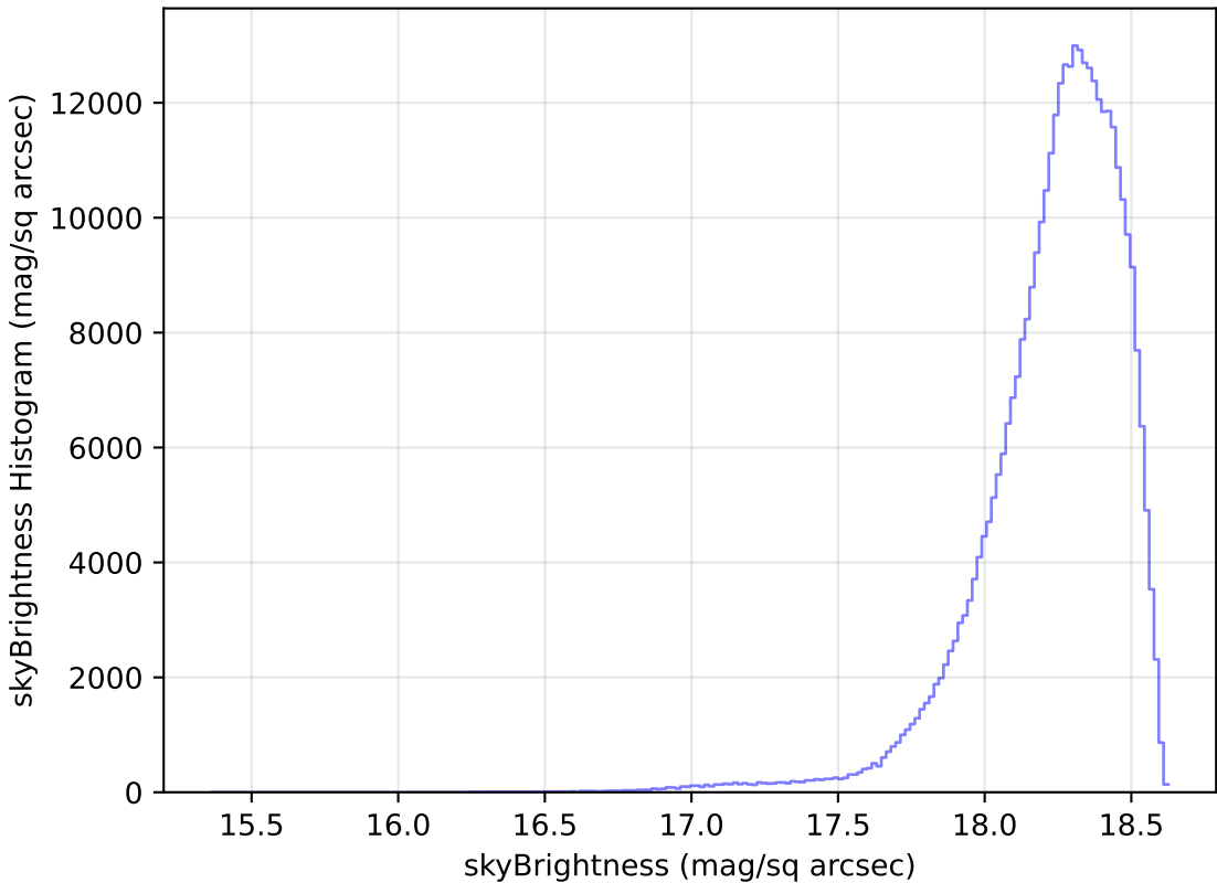
baseline_v3.3_10yrs All sky y band: skyBrightness Histogram
